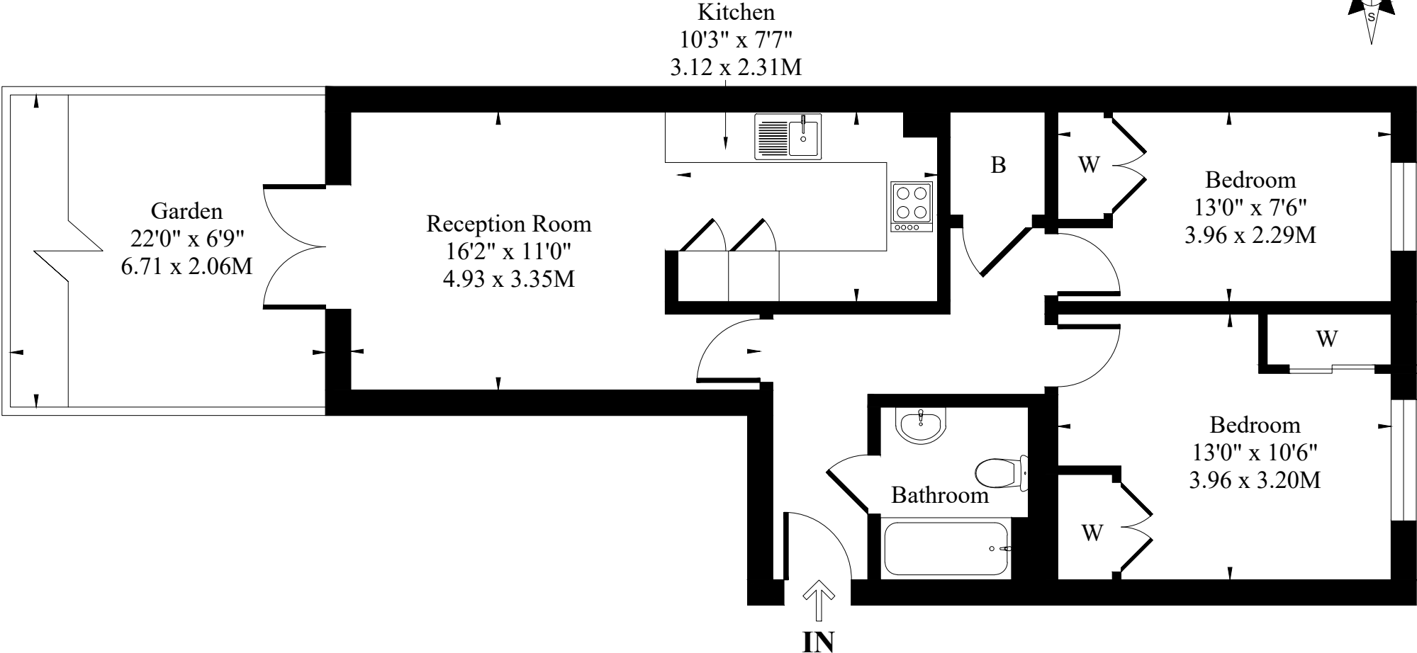
Floor Plan
